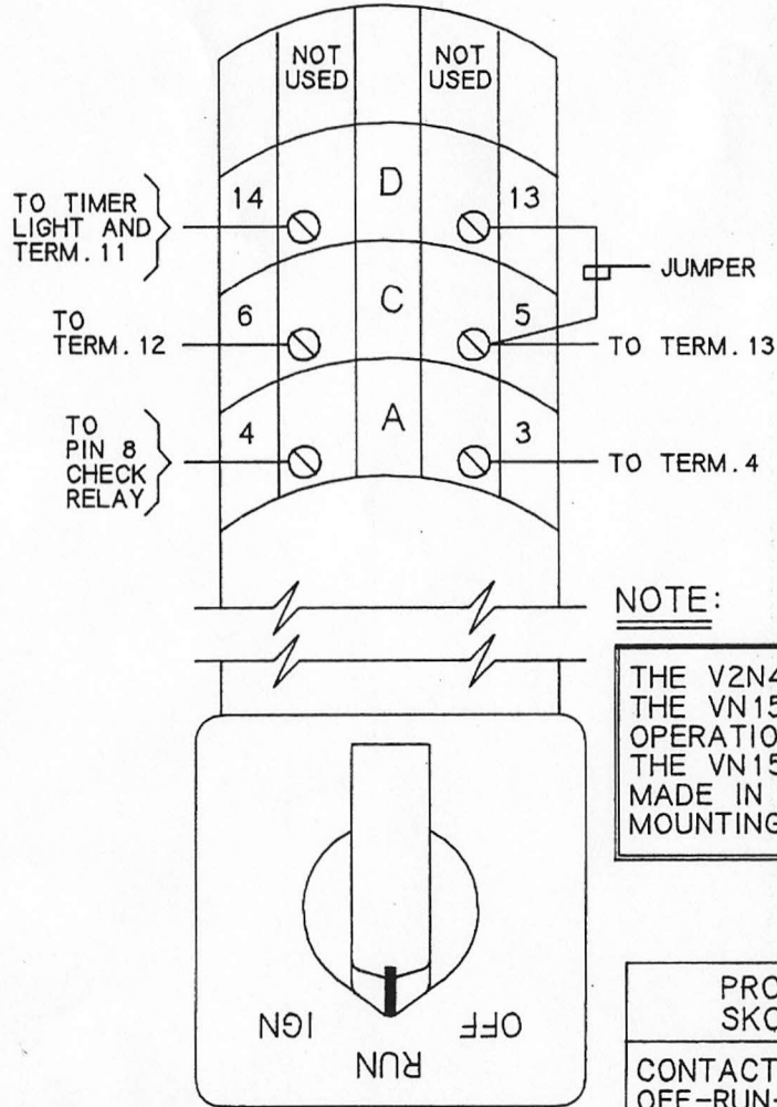
SWITCH NO. V2N4T911-UL THREE POSITION OPERATOR SPRING RETURN FROM RIGHT TO CENTER.
