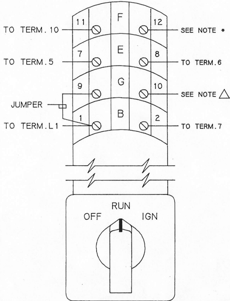
SWITCH NO. V2N4T911-UL THREE POSITION OPERATOR SPRING RETURN FROM RIGHT TO CENTER.
